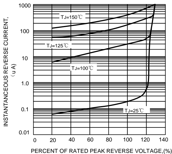
FIG.5-TYPICAL REVERSE CHARACTERISTICS
