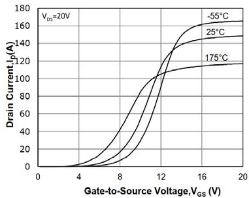
Fig 6: Transfer Characteristic
