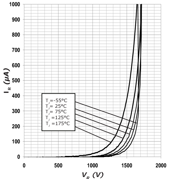
Figure 2. Reverse Characteristics
