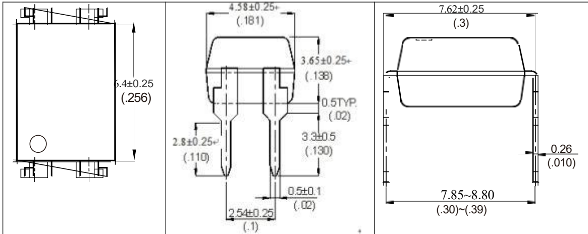
4-pin DIP
