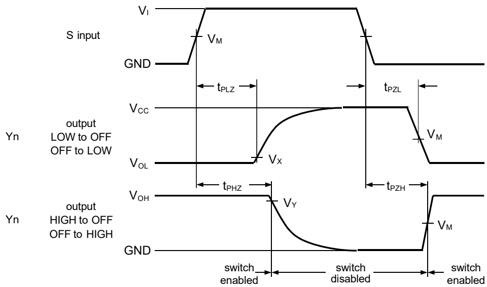
Logic levels: V_{OL} and V_{OH} are typical output voltage levels that occur with the output load. Figure 13. Enable and disable times
