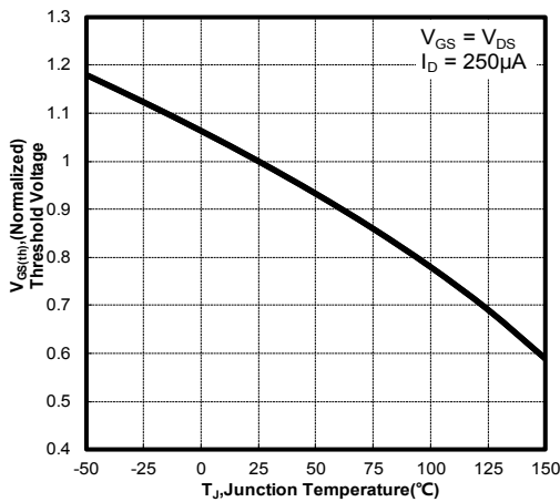
Gate Threshold Voltage V_{TH}=f(T_j); I_D=250\mu A
