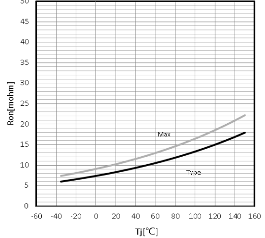
Drain-source on-state resistance R_{DS(on)}=f(T_j); I_D=20A; V_{GS}=10V
