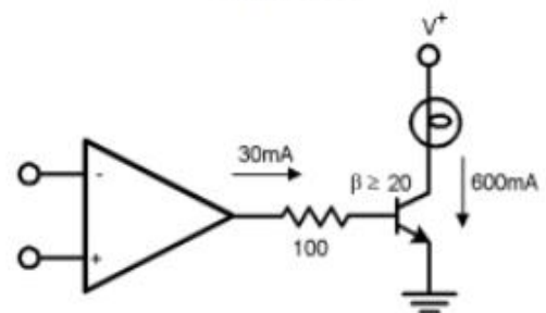
Lamp Driver
