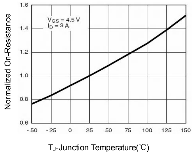
Figure 8 Drain-Source On-Resistance
