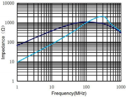
CMF9070-132-2P-T
