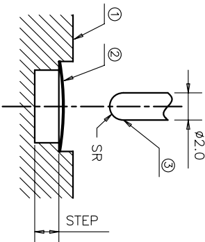
Fig.1. MEASURING METHOD
