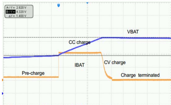
Charge Curve
