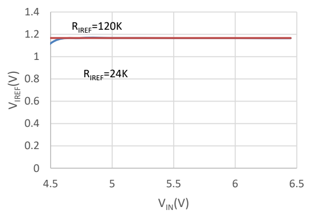
V_{\text{IREF}} \text{ vs } V_{\text{IN}}
