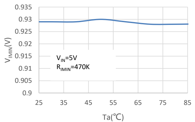
V_{IMIN} vs T_a
