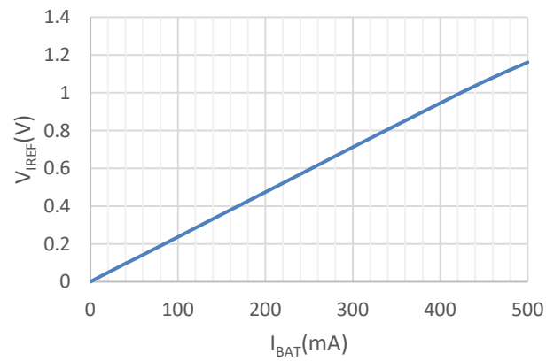
V_{\text{IREF}} \text{ vs } I_{\text{BAT}}
