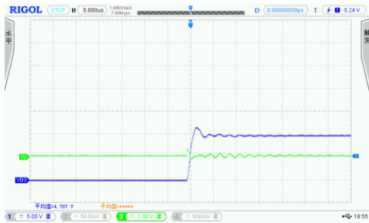
CH1:V IN
