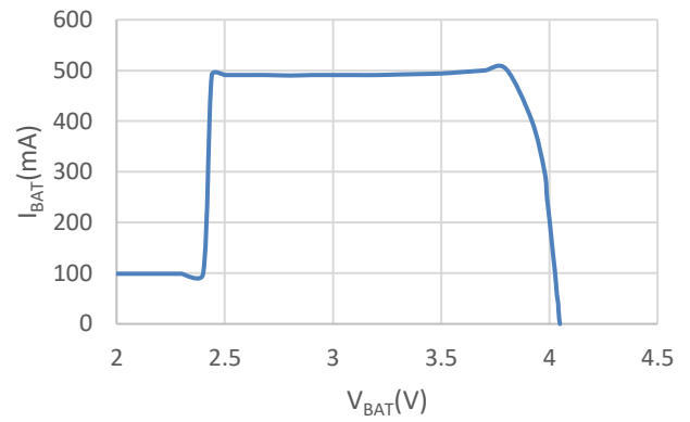
Charge Curve
