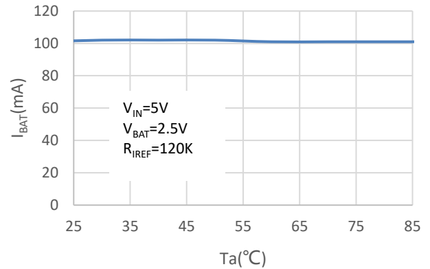
I_{BAT} vs T_a
