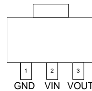
SOT89-3L (Top View)
