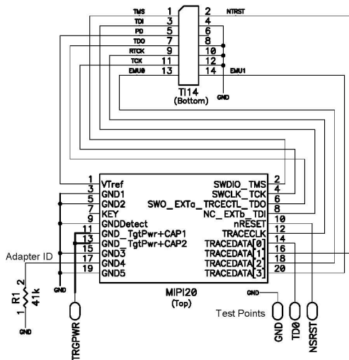
Figure 7: Diagram of the ADA-MIPI20-TI14 adapter
