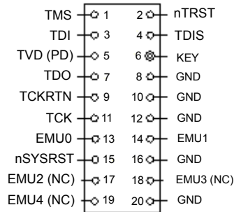
Figure 13: Pinout of the target cTI20 JTAG header
