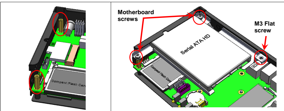
Fig. 9-3 Remove two motherboard screws and fasten two standoffs
