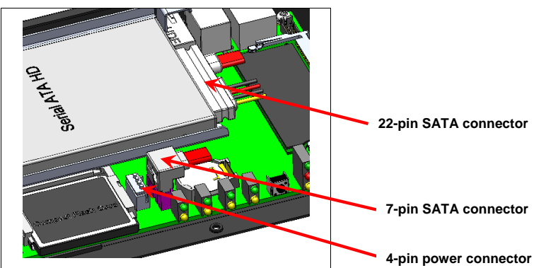
Fig. 9-5 Plug SATA cable
