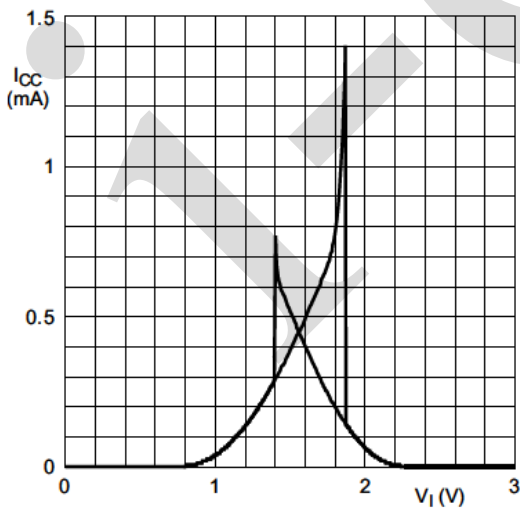
图8 典型AiP74AHC1G14传输特性; V_{CC}=3.0V
