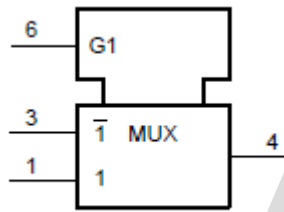
Figure 2. IEC logic symbol
