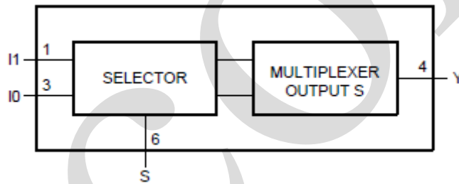
Figure 3. Logic diagram
