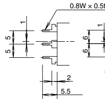
[PC Board Terminal]
