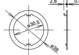
OGL-31 Anti-Rotation Ring
