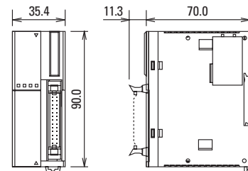
FC4A-D20K3, FC4A-D20S3
