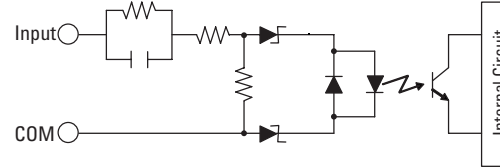
FC4A-N08A11
