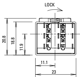
[3PDT]
