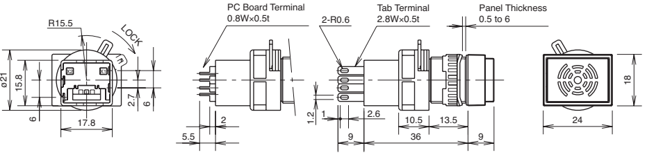
Solder/Tab Terminal
