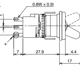
[Solder/Tab Terminal]
