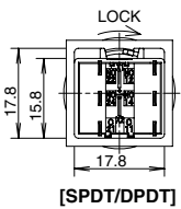
[SPDT/DPDT]
