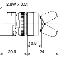
[Solder/Tab Terminal]
