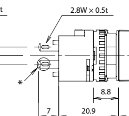
[Solder/Tab Terminal]
