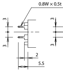
[PC Board Terminal]
