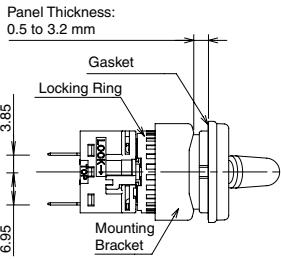
[PC Board Terminal]
