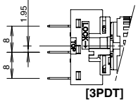
[3PDT]
