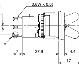
[Solder/Tab Terminal]
