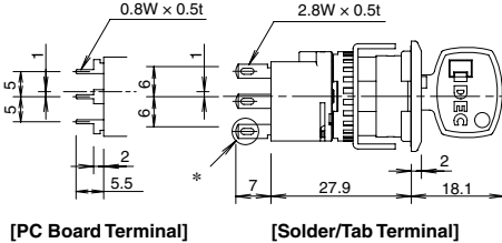
[PC Board Terminal]
