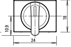
[Lever Operator]
