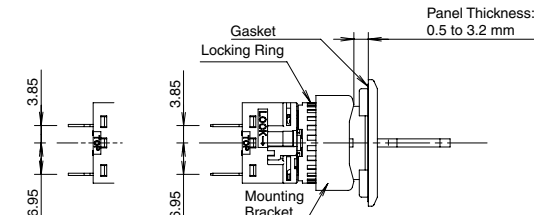
[SPDT/DPDT]
