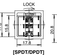
[SPDT/DPDT]
