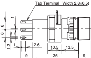
Solder/Tab Terminal
