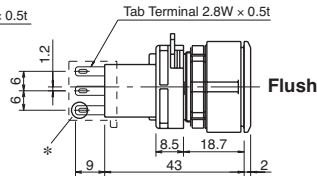
Solder/Tab Terminal
