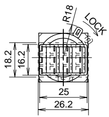
Solder/Tab Terminal
