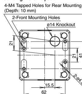
Mounting Hole Layout
