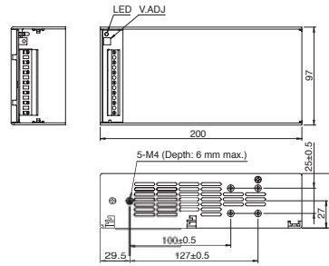
PS3L-E (100W)
