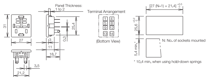
SH2B-51
