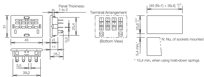
SH4B-51
