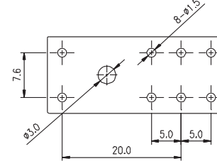
SQ2V-63 PCB Pin Layout
