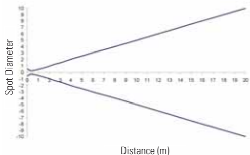
Light Spot Dimension - Laser Polarized Retro-reflective
