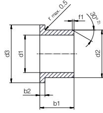
3) Thickness < 0.6mm: chamfer = 20°
