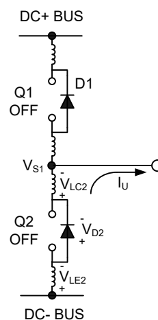
Figure 13 VS negative
