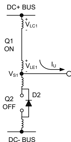
Figure 12 VS positive
