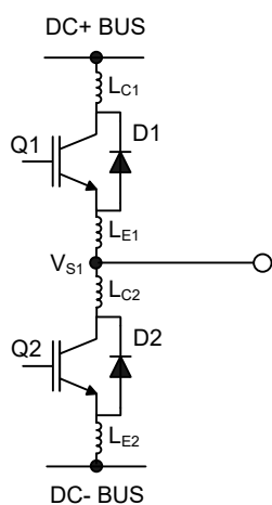
Figure 11 Parasitic Elements
