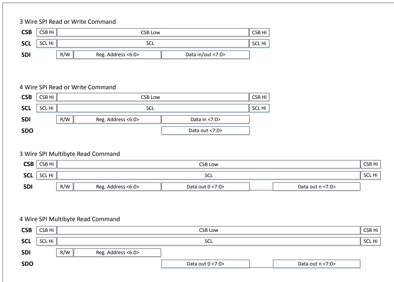
Figure 12 SPI write, read protocol diagrams
