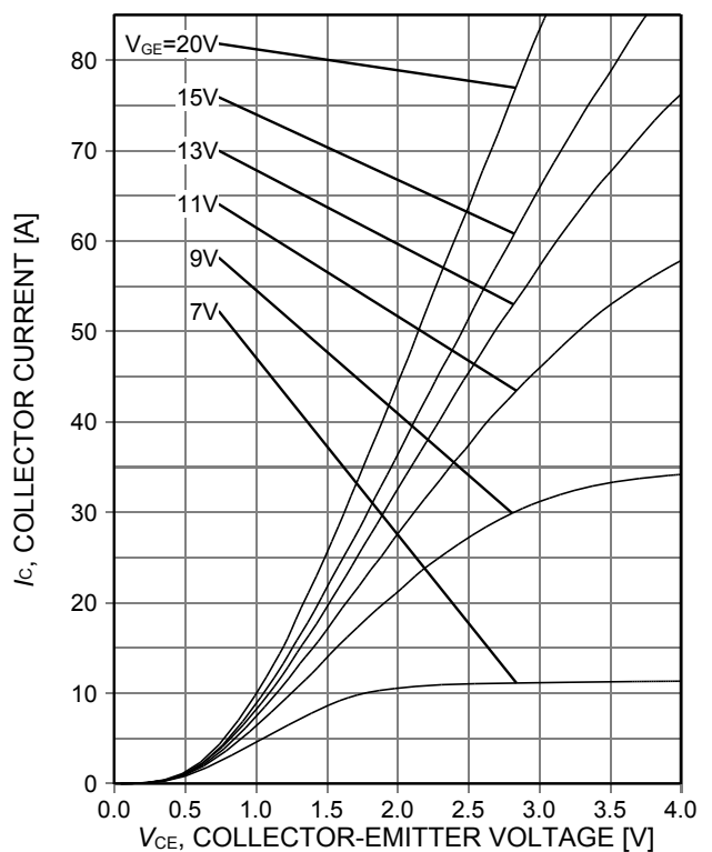
Figure 4. Typical output characteristic ( T_j = 175^\circ\text{C} )
