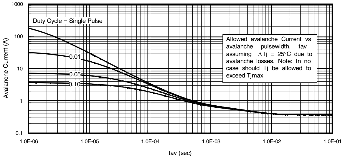
Fig 15. Typical Avalanche Current Vs.Pulswidth
