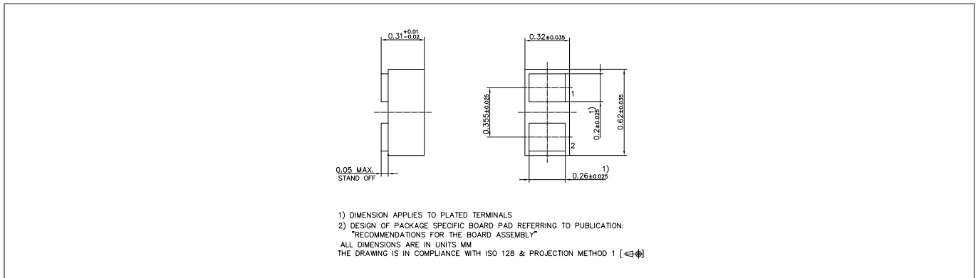
Figure 8 Package outline
