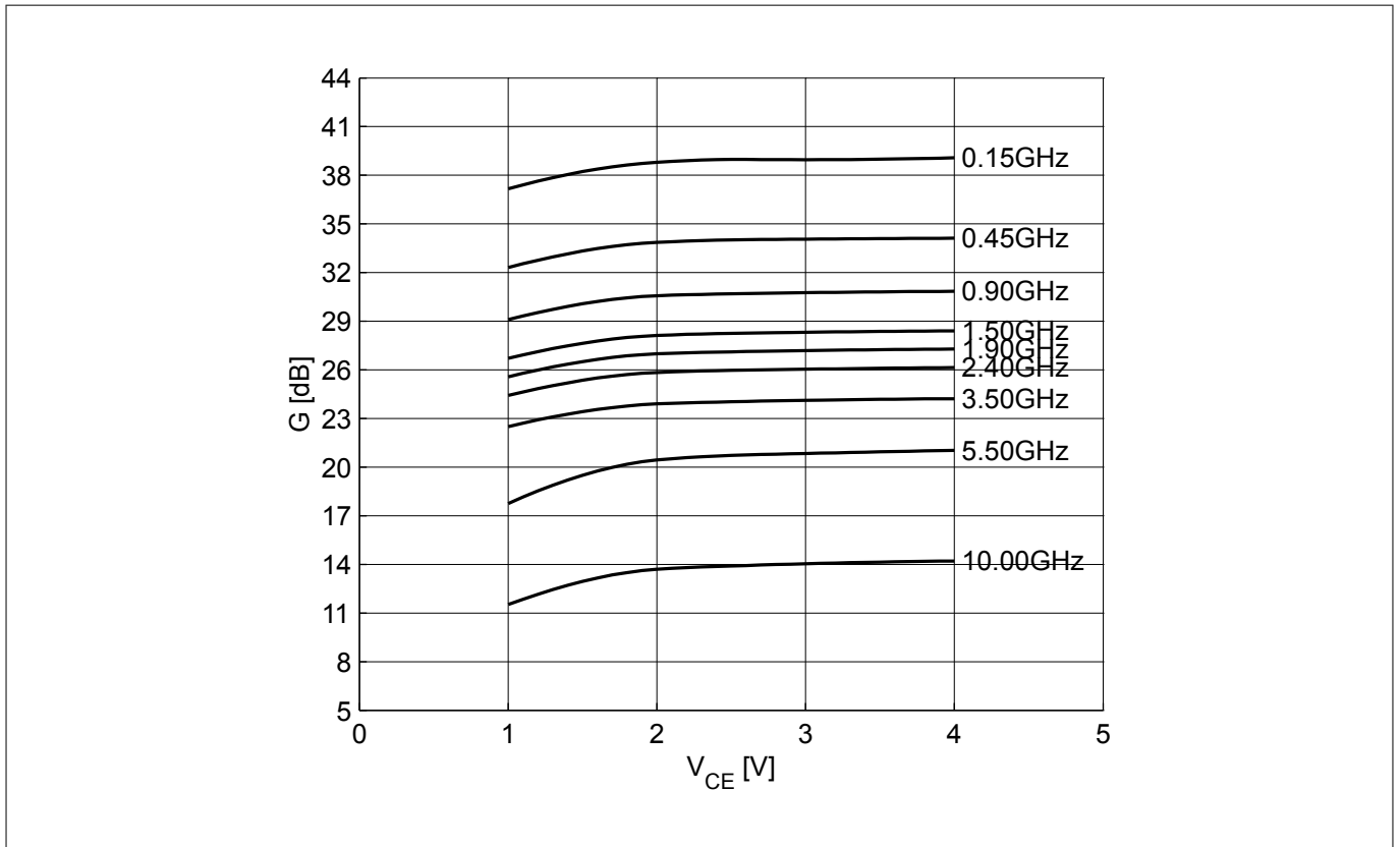
Figure 13 Maximum power gain G_{max} = f(V_{CE}) , I_C = 25\text{ mA} , f = parameter in GHz
