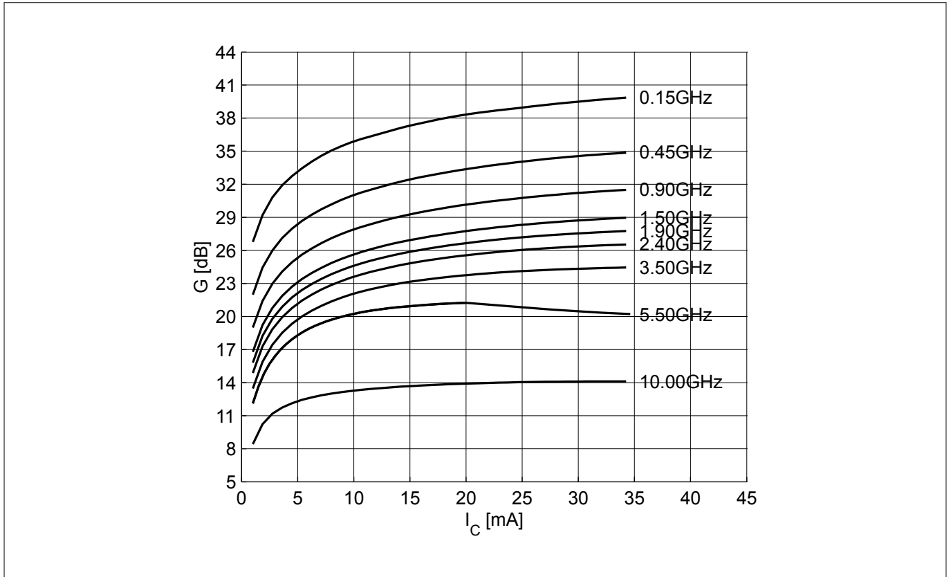
Figure 12 Maximum power gain G_{max} = f(I_C) , V_{CE} = 3\text{ V} , f = parameter in GHz
