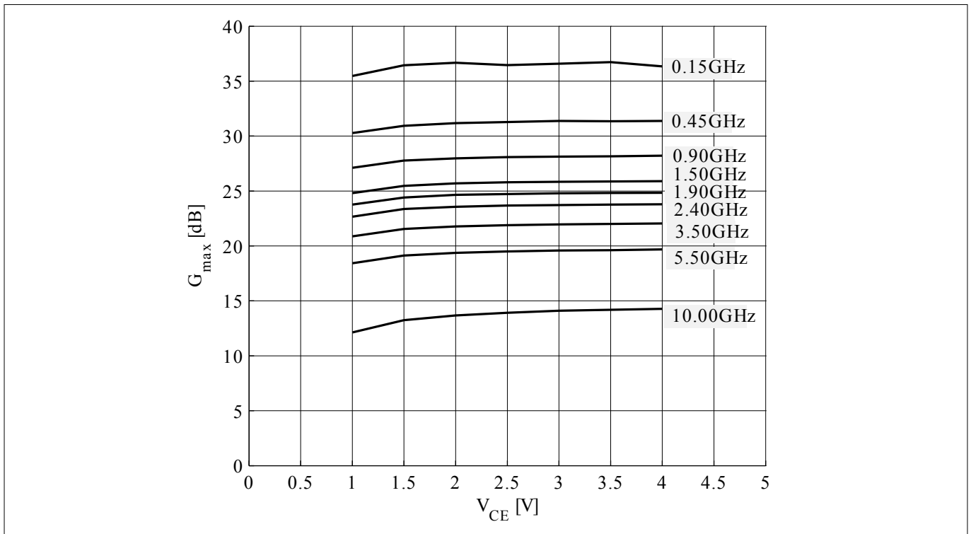
Figure 15 Maximum power gain G_{max} = f(V_{CE}) , I_C = 15\text{ mA} , f = parameter in GHz
