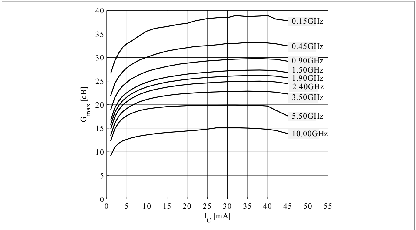
Figure 14 Maximum power gain G_{max} = f(I_C) , V_{CE} = 3\text{ V} , f = parameter in GHz
