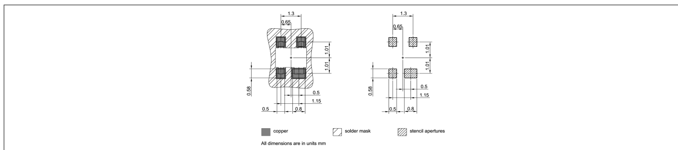
Figure 23 Foot print
