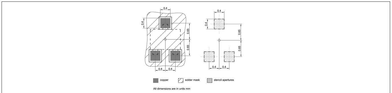
Figure 16 Foot print
