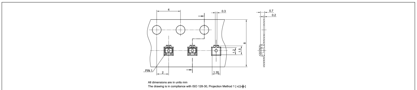
Figure 18 Tape information
