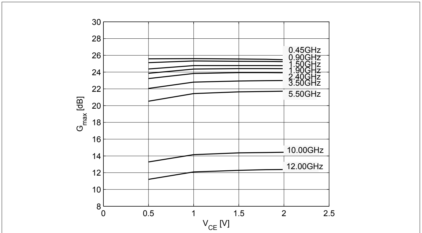
Figure 13 Maximum power gain G_{max} = f(V_{CE}) , I_C = 15\text{ mA} , f = \text{parameter}
