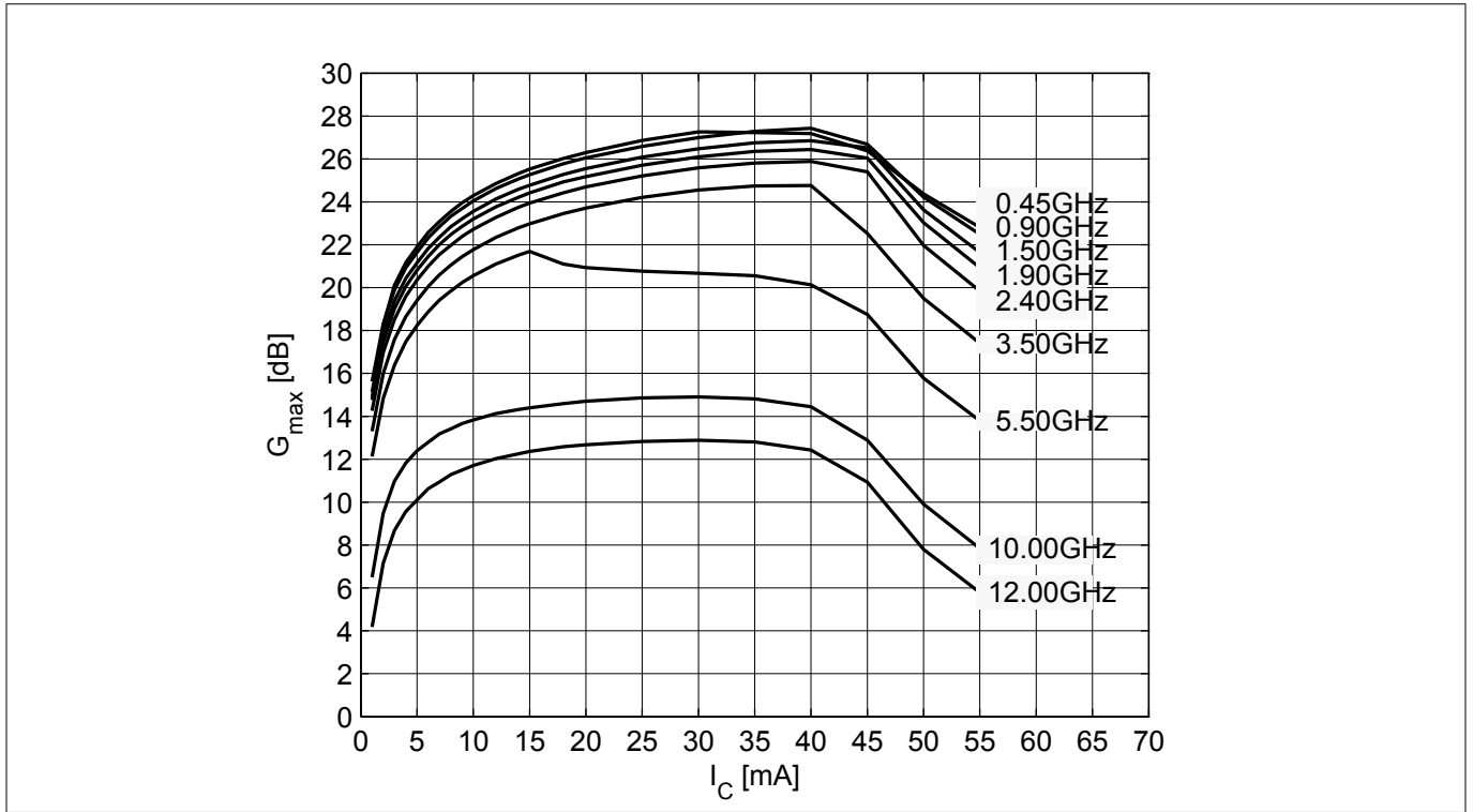
Figure 12 Maximum power gain G_{max} = f(I_C) , V_{CE} = 1.8\text{ V} , f = \text{parameter}
