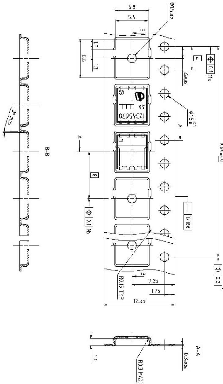
Dimension in mm
