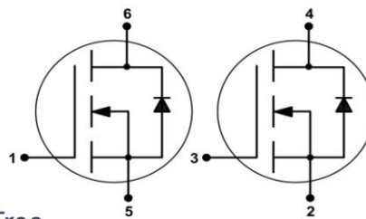
PG-TSOP6
