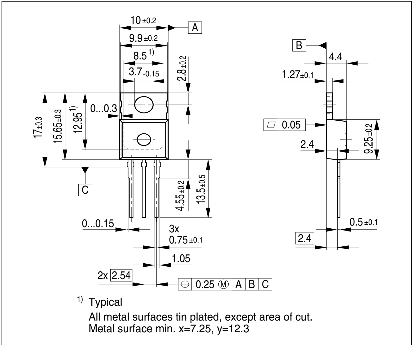
Figure 1 PG-T0220-3-1
