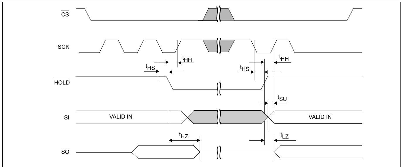
Figure 17 \overline{HOLD} timing
