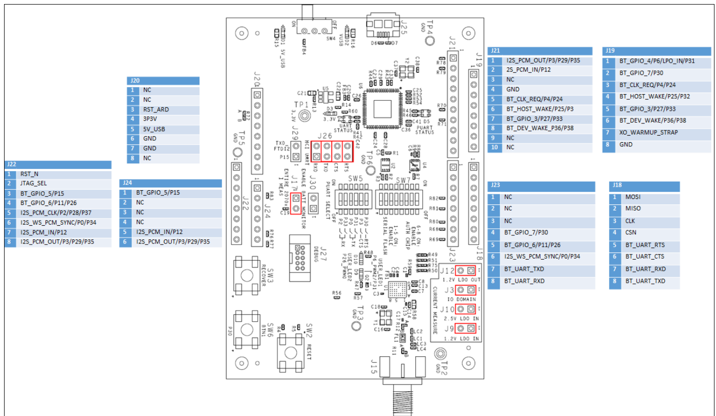
Figure 1-2 shows the pins connected to the user accessible headers on the board.
